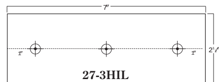
2 1/2" x 7" Three Holes In Line – Countersunk
