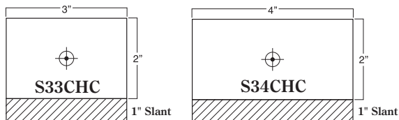
3" x 3" One Hole – Countersunk
