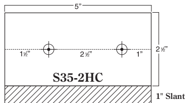
3 1/2" x 5" Two Holes Offset – Countersunk
