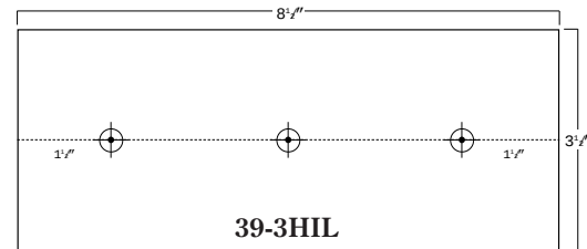
39-3HIL 3 1/2" x 8 1/2" Three Holes In Line - Countersunk
