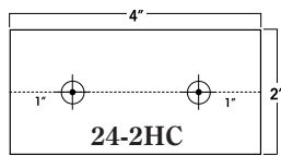
24-2HC 2" x 4" Two Holes In Line - Countersunk
