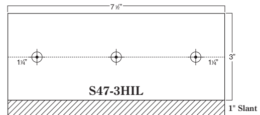
4" x 7 1/2" Three Holes In Line – Countersunk
